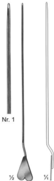
05-169 LOCKHART-MUMMERY 165 mm
